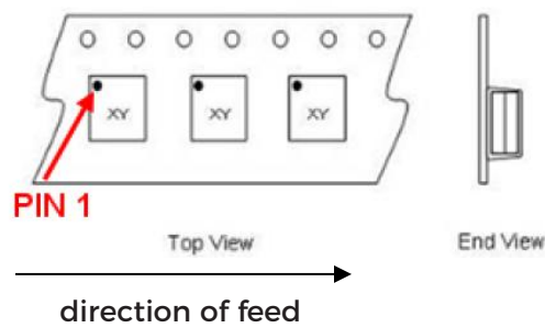
Fig 2. Product orientation in carrier tape
