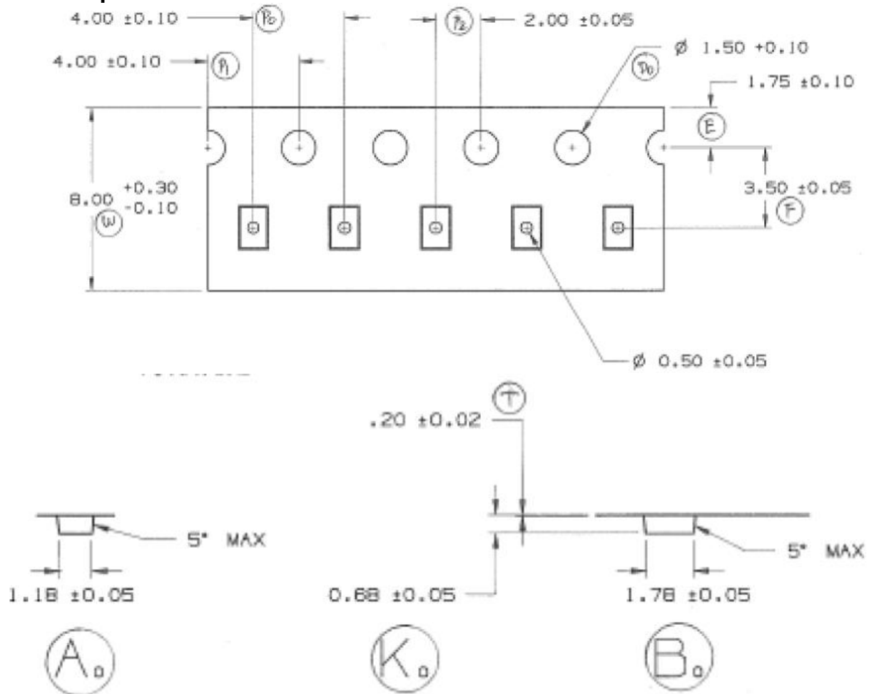
Fig 3. Carrier tape dimensions
